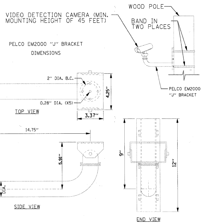
TEMPORARY CAMERA MOUNTING DETAILS (NOT TO SCALE)
