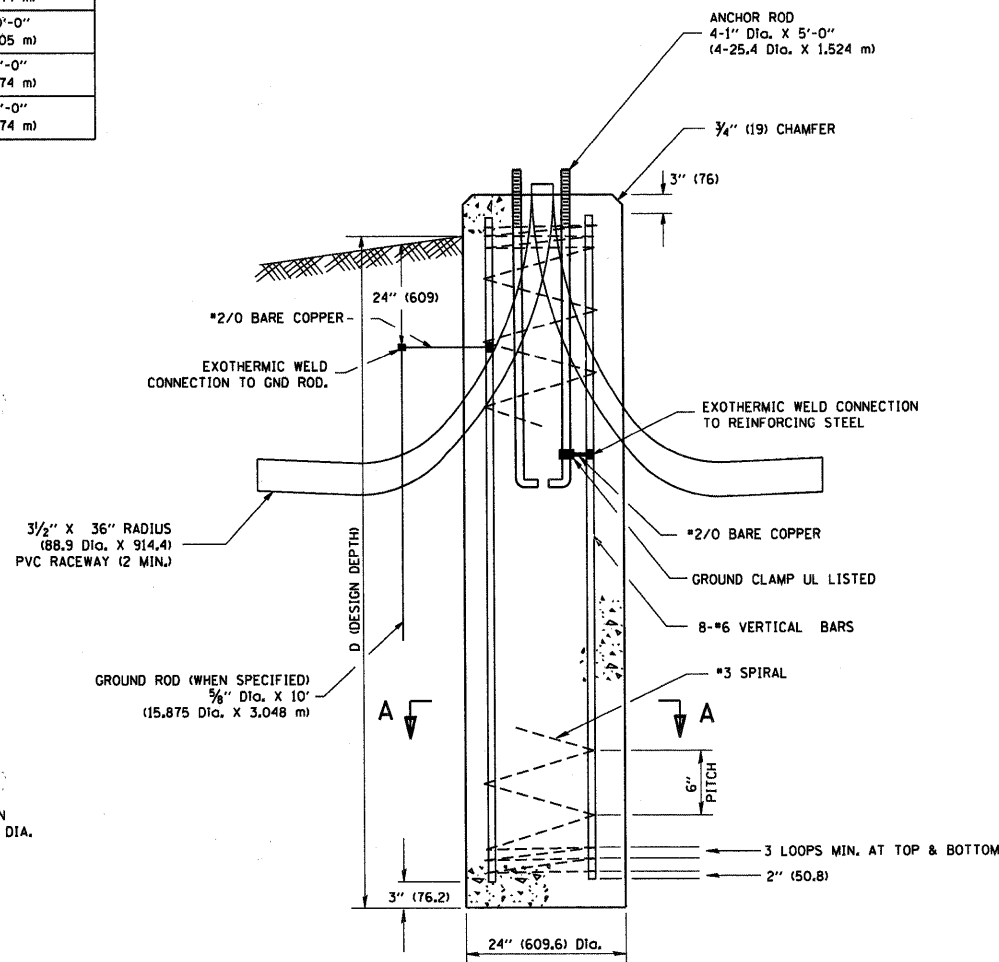
FOUNDATION DETAIL
