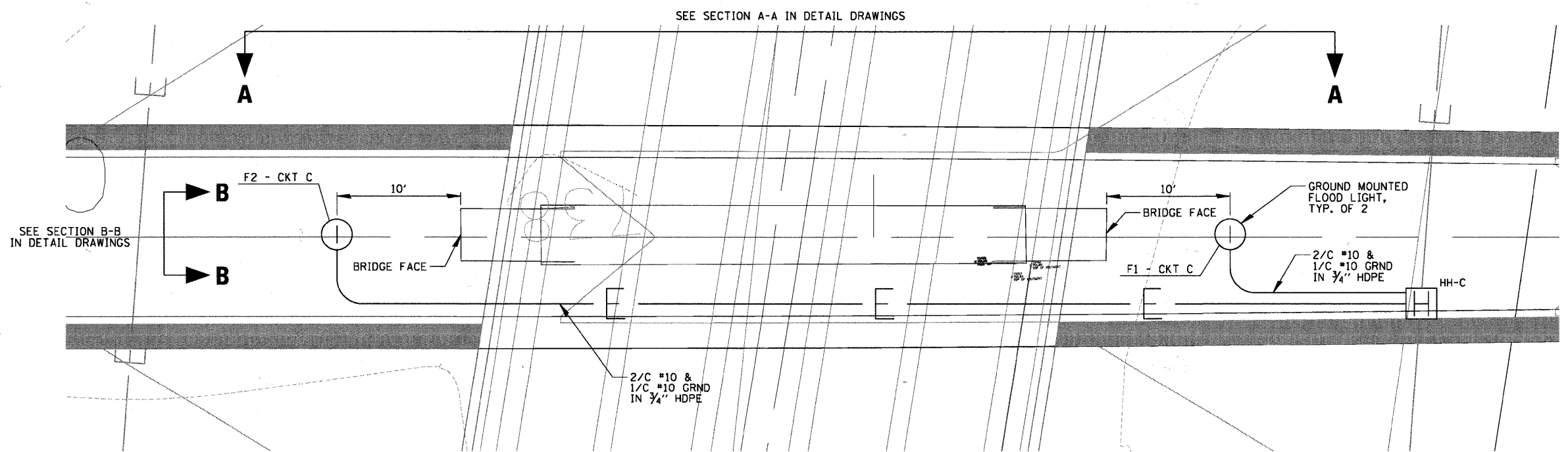
ENLARGED LIGHTING PLAN N.T.S.
