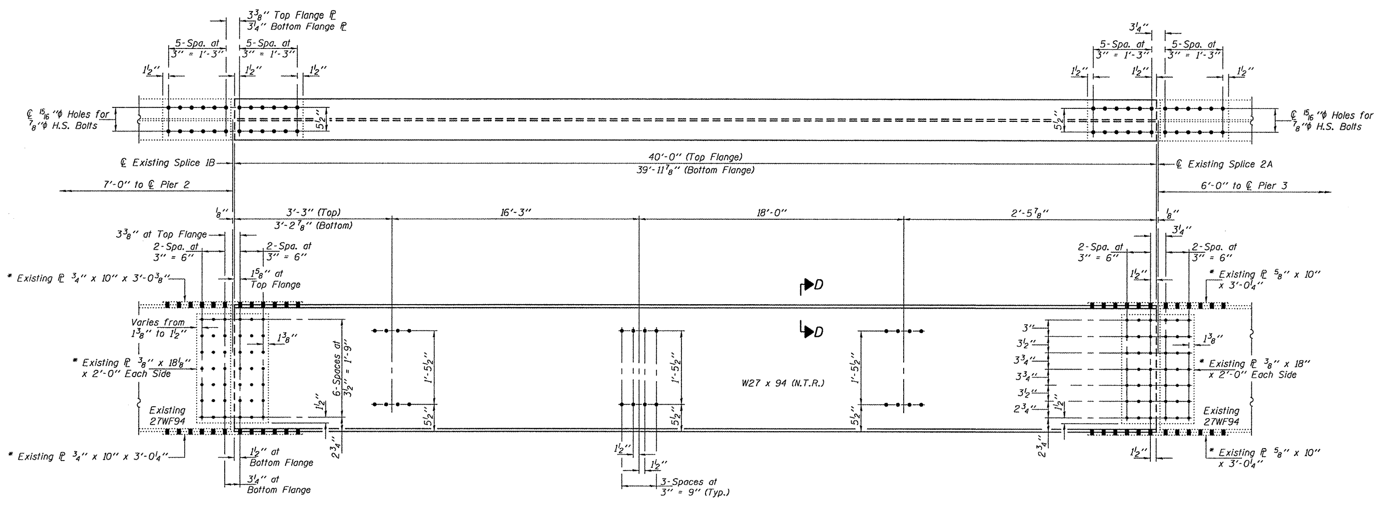
ELEVATION BEAM 5 SPAN 3
