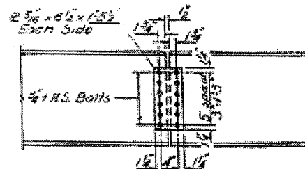
DETAIL OF SPLICE AT BENTS 3 & 6
