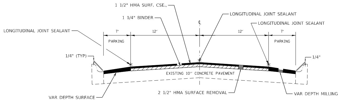
TYPICAL SECTION 4 STA 22+82 TO STA 0+00
