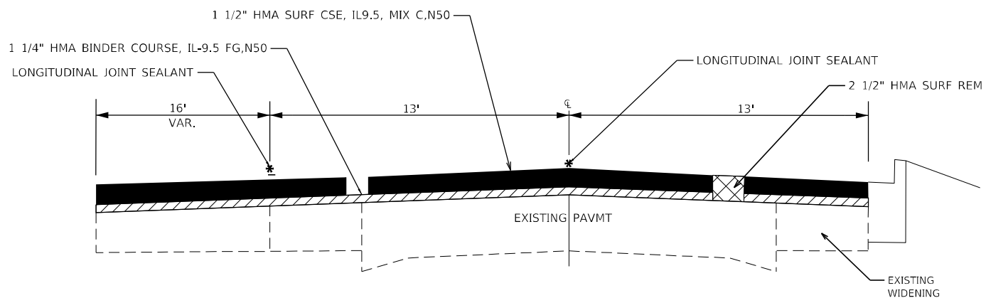
TYPICAL SECTION 5 STA 25+77 TO STA 22+82
