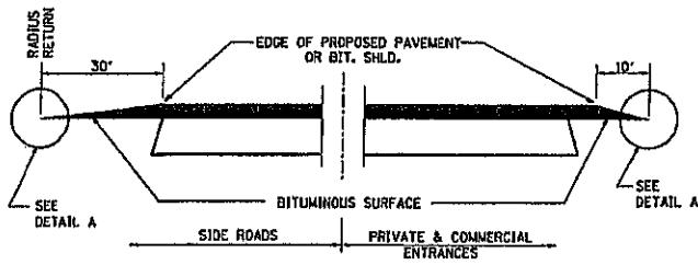
SECTION A-A DETAILS AT ENTRANCES & SIDE ROADS
