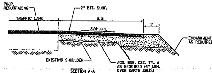
SECTION A-A MAILBOX TURNOUT DETAILS
