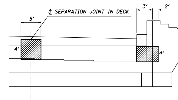
SOUTHEAST WINGWALL AND ABUTMENT (Looking East) SN 057-0048 (WB)
