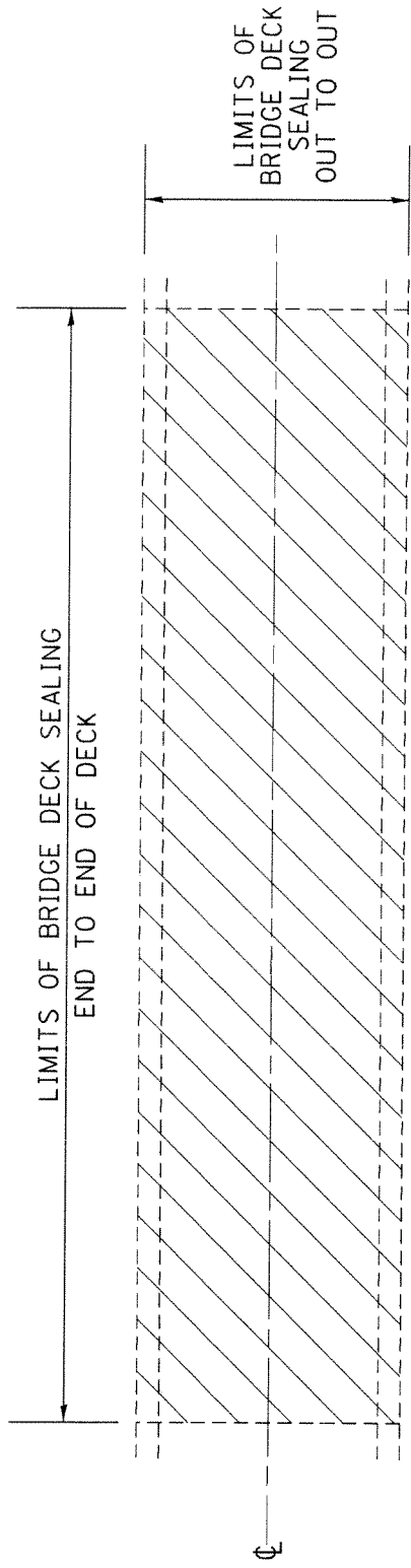
PLAN VIEW
