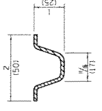
SECTION E-E
