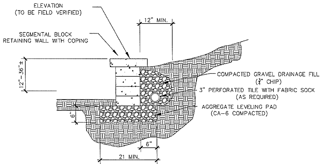
SEGMENTAL CONCRETE BLOCK WALL DETAIL N.T.S
