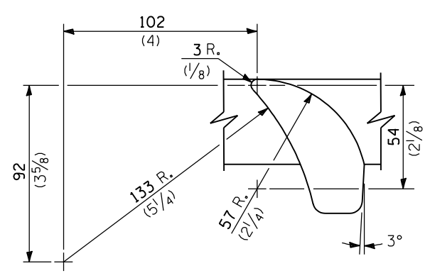
VANE DETAILS
