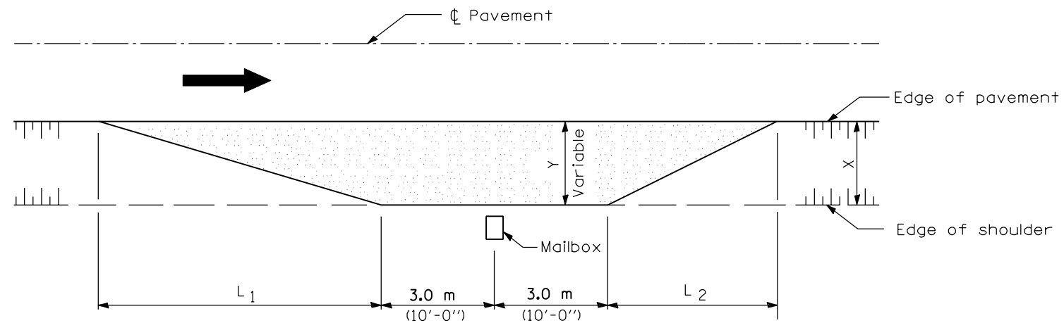
TYPICAL APPLICATION
