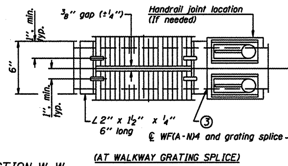
SECTION W-W
