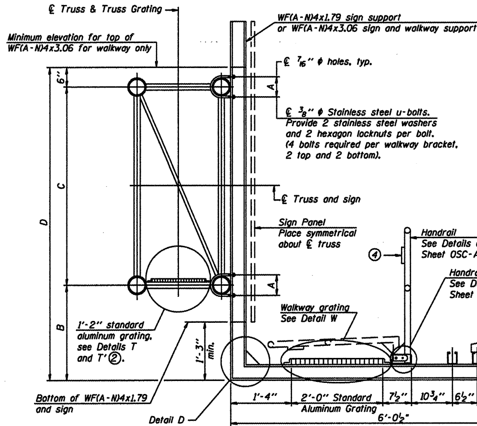
SECTION B-B
