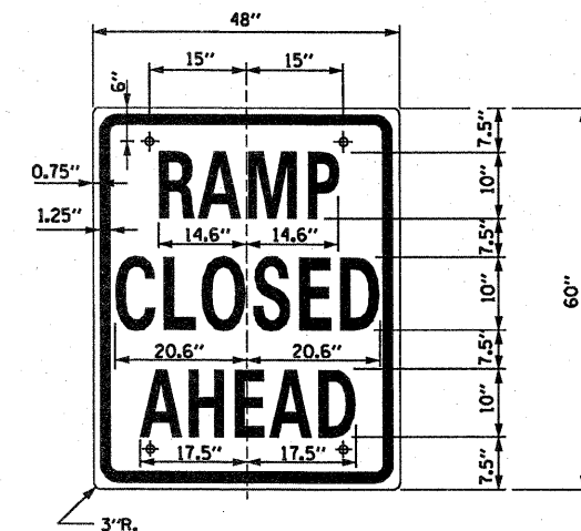
SIGN TS-9
