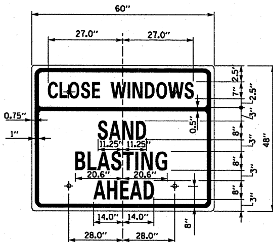
SIGN TS-10
