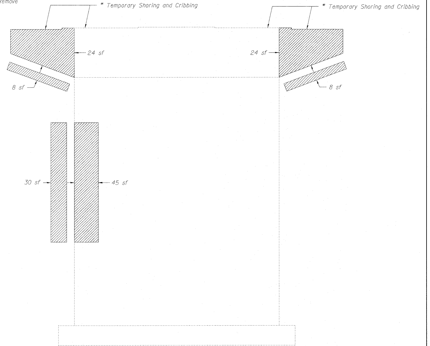
PIER 20 (South Face)
