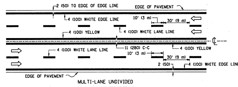
MULTI-LANE UNDIVIDED
