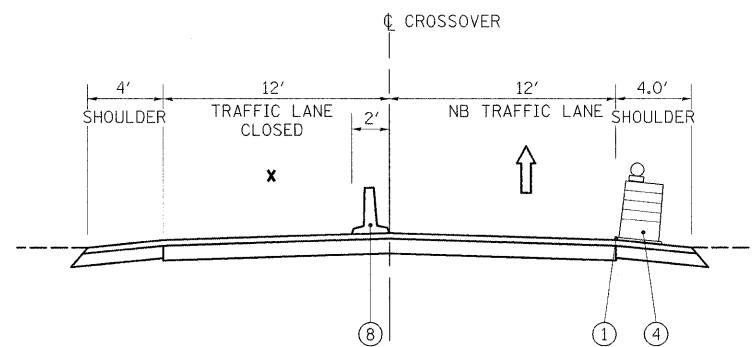
CROSSOVER TYPICAL SECTION - STAGE II SOUTH BOUND PEAK (SECTION LOOKING NORTH) STA. 33+50 TO STA. 42+50 STA. 76+50 TO STA. 87+50
