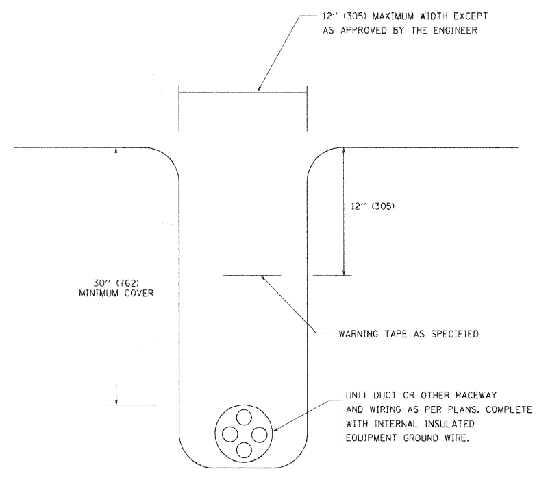
TYPICAL WIRING IN TRENCH DETAIL N.T.S.
