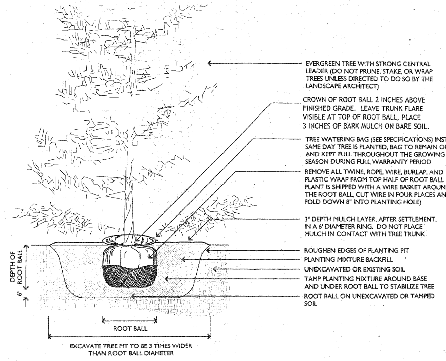
2 EVERGREEN TREE INSTALLATION DETAIL SCALE: 1/2"=1'-0"
