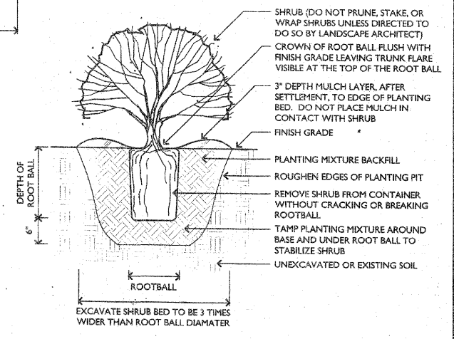
5 CONTAINER SHRUB INSTALLATION DETAIL SCALE: 1"=1'-0"
