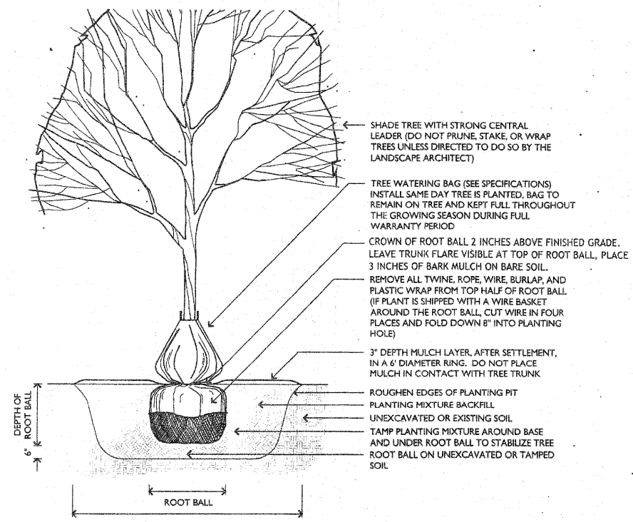
1 DECIDUOUS TREE INSTALLATION DETAIL SCALE: 1/2"=1'-0"
