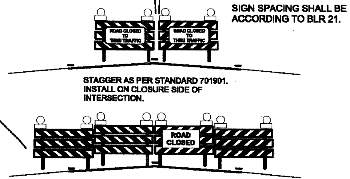
TRAFFIC CONTROL CLOSURE AT STRUCTURE.
