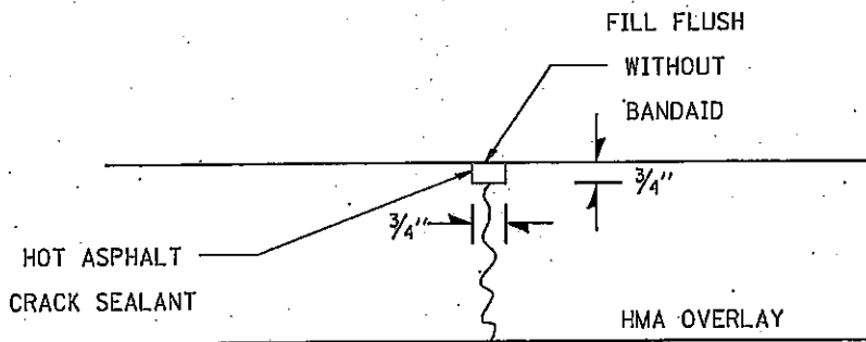
PAVEMENT CROSS-SECTION
