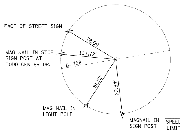
TIE POINT CUT "X" PT STATION 138+50.58
