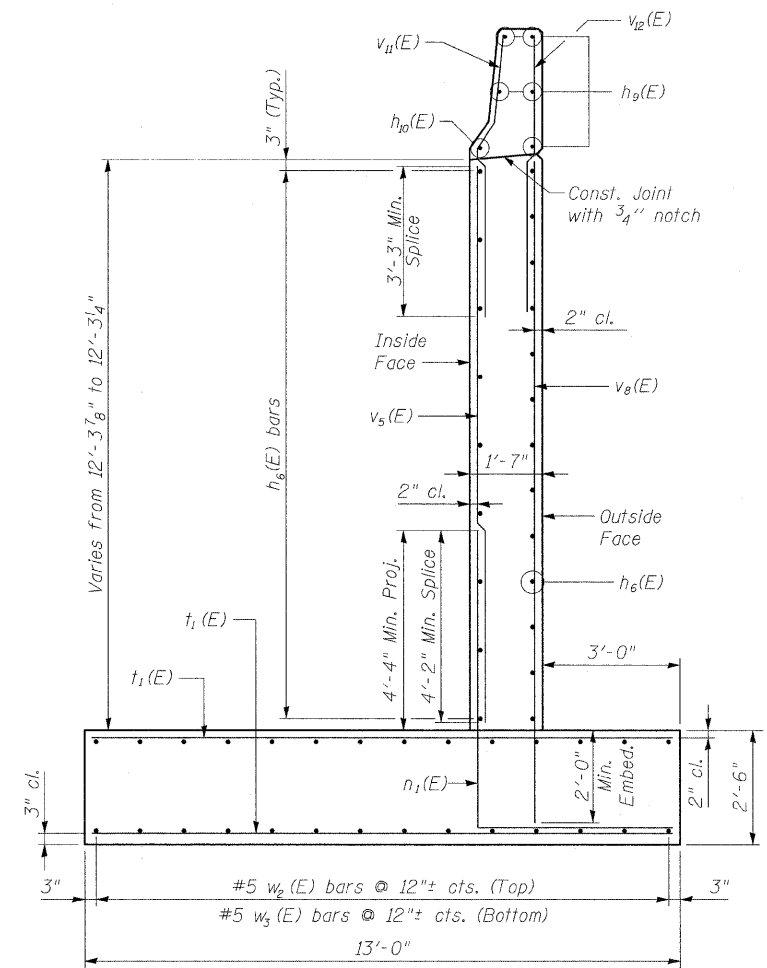
SECTION C-C
