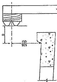
GUARDRAIL PLACED BEHIND CURB D = 0 constructible to 300 (12) maximum
