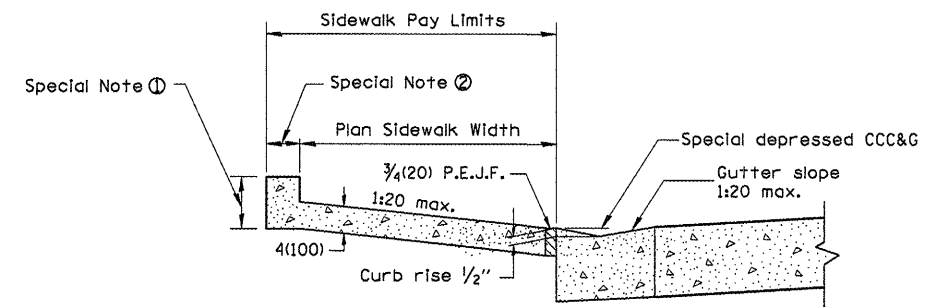
SEC. E-E
