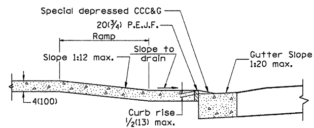
SEC. G-G
