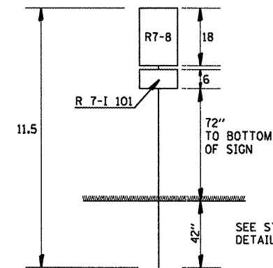
SIGN POST DETAILS
