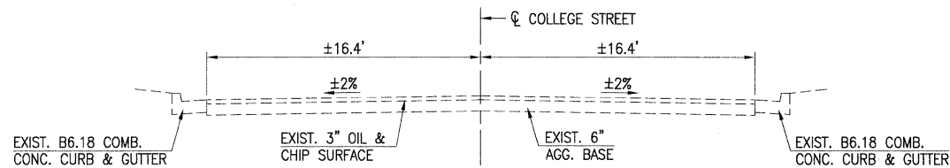
COLLEGE STREET EXISTING TYPICAL SECTION STA. 60+32.0± TO STA. 62+95.00
