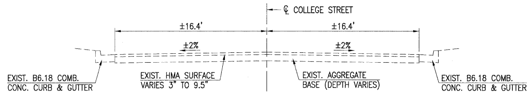
COLLEGE STREET EXISTING TYPICAL SECTION STA. 59+83.00 TO STA. 60+32.0±
