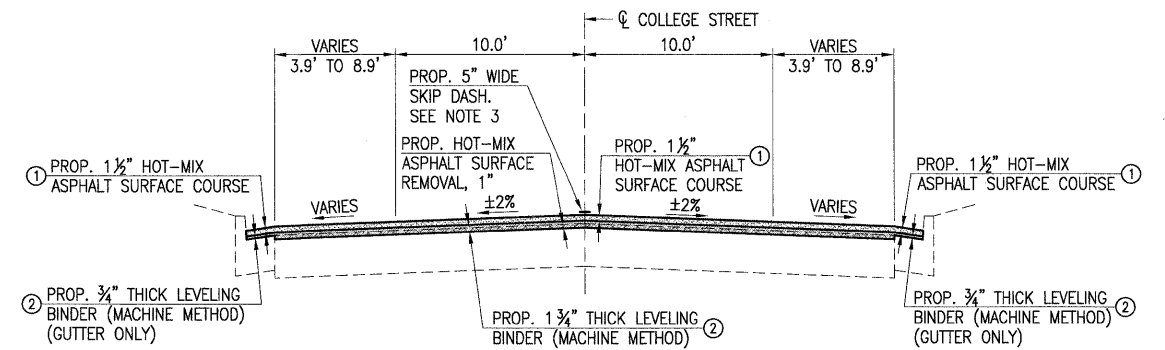
COLLEGE STREET PROPOSED TYPICAL SECTION STA. 50+20.30 TO STA. 54+79.30
