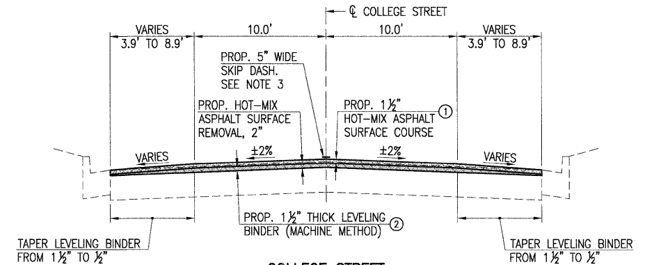
COLLEGE STREET PROPOSED TYPICAL SECTION STA. 54+79.30 TO STA. 60+32.0±
