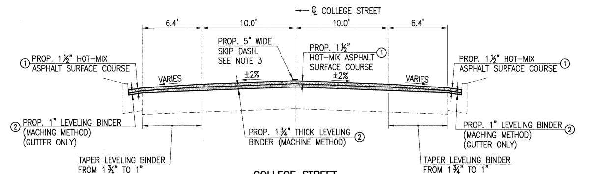
COLLEGE STREET PROPOSED TYPICAL SECTION STA. 60+32.00± TO STA. 62+95.00
