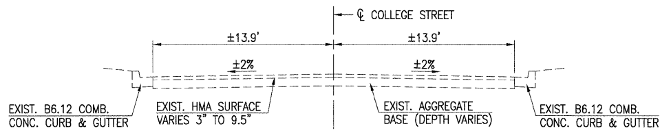
COLLEGE STREET EXISTING TYPICAL SECTION STA. 50+44.00 TO STA. 59+83.00
