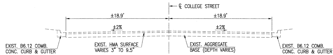
COLLEGE STREET EXISTING TYPICAL SECTION STA. 50+20.30 TO STA. 50+44.00
