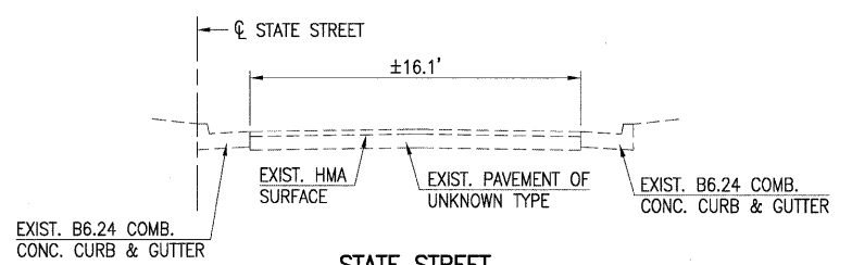
STATE STREET EXISTING TYPICAL SECTION STA. 31+53.20 TO STA. 31+95.80
