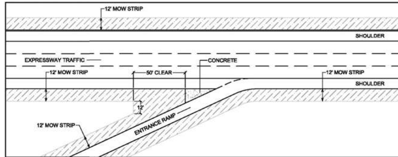
Mowing Detail #3
