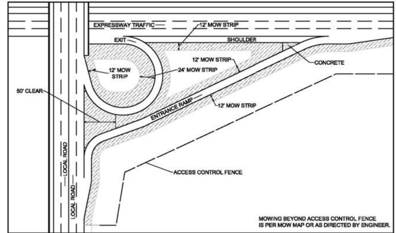
Mowing Detail #2
