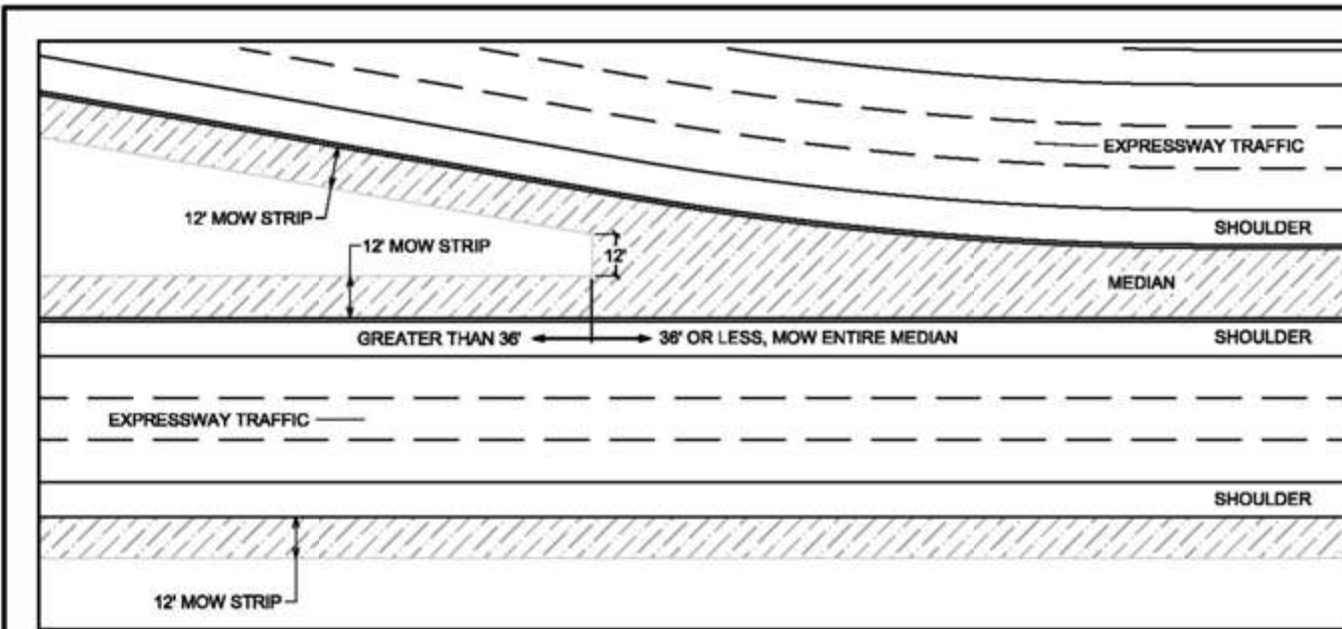
Mowing Detail #1
