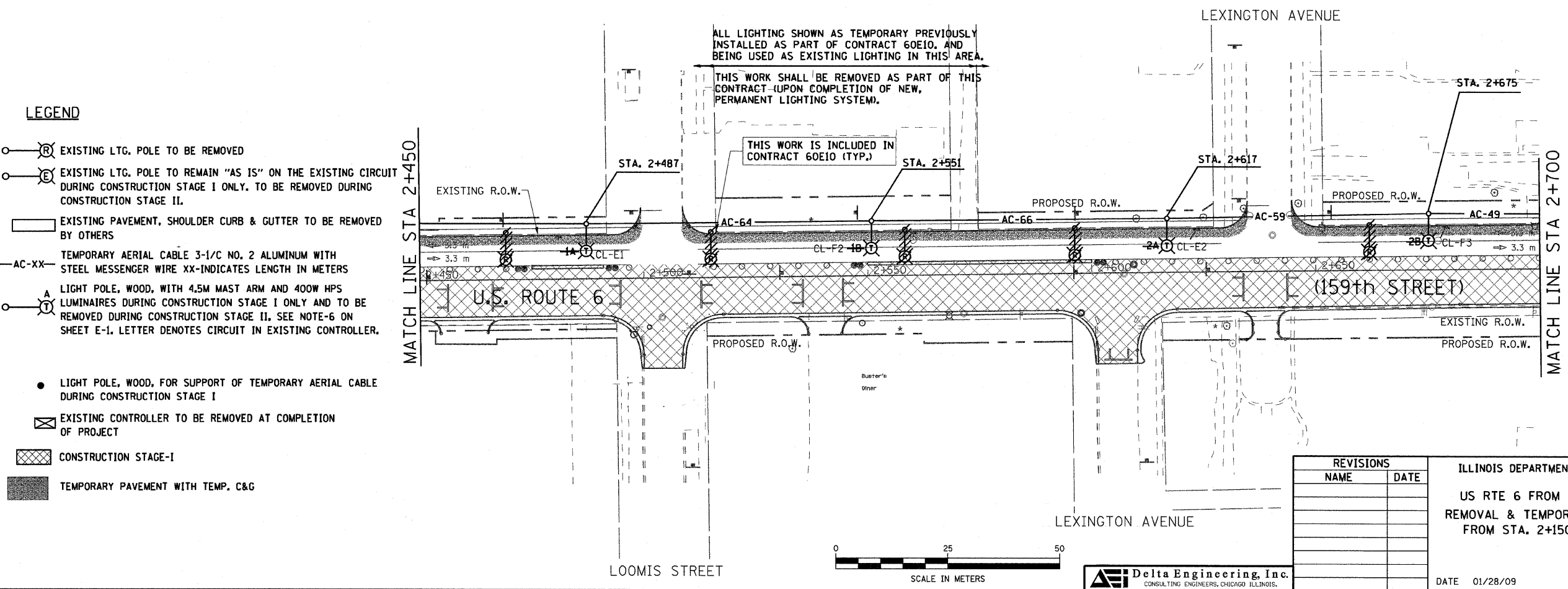
DRAWING No. E-5
