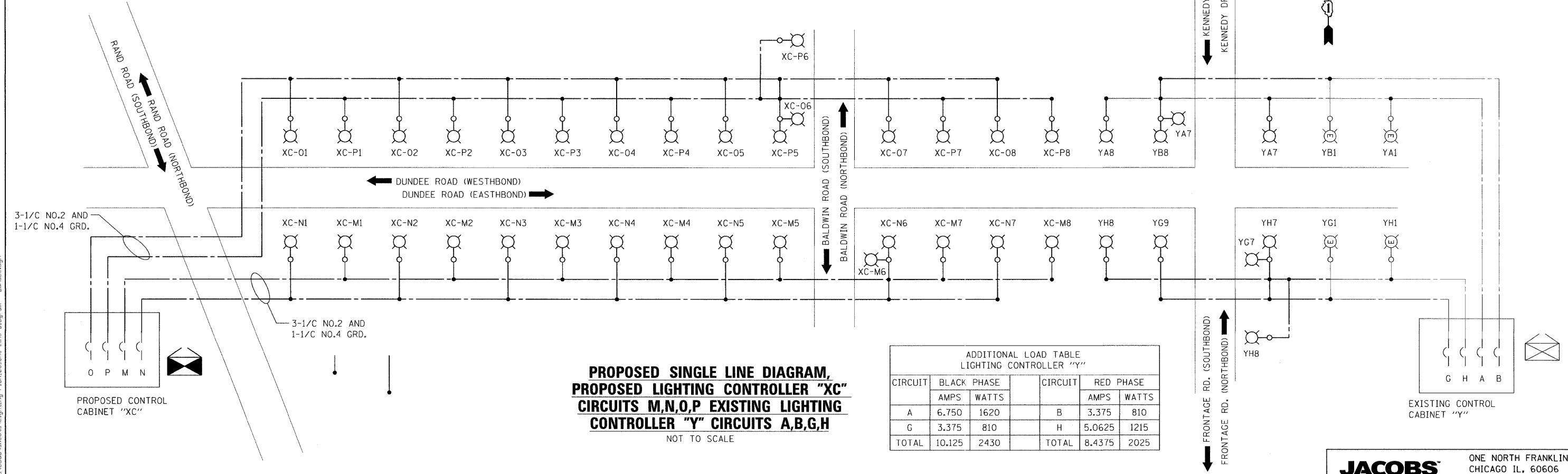
PROPOSED CONTROL CABINET "XC"
