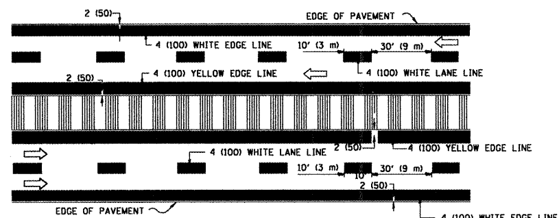
MULTI-LANE DIVIDED WITH MOUNTABLE MEDIUM
