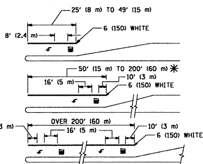
TYPICAL PAINTED MEDIUM MARKING
