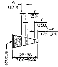
REFLECTORIZED CONE
