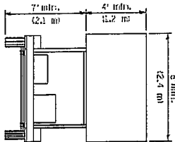
TYPE C TRAILER MOUNTED
