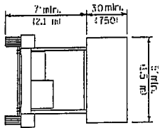
TYPE B ROOF OR TRAILER MOUNTED
