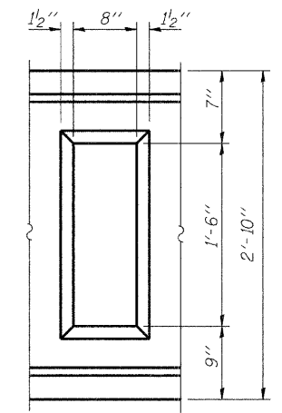
WINDOW DETAIL
