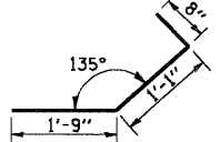
#4 f BAR FRONTWALL
