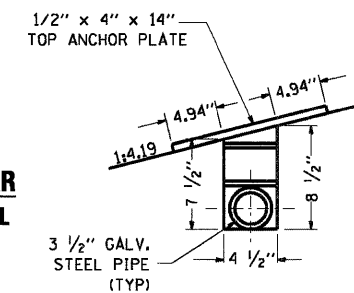
NOTCH DETAIL
