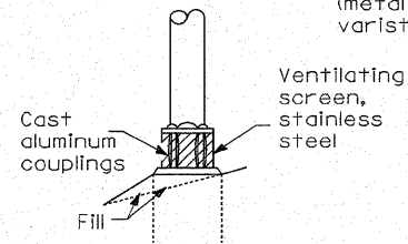
BREAKAWAY COUPLING
