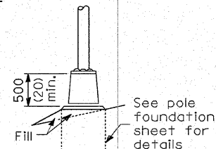
TRANSFORMER BASE
