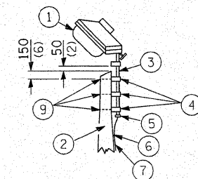
TENON
