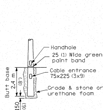
BUTT BASE
