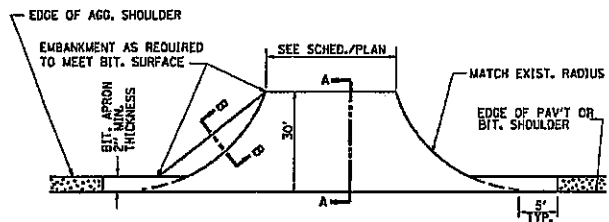
PLAN AT SIDE ROADS
