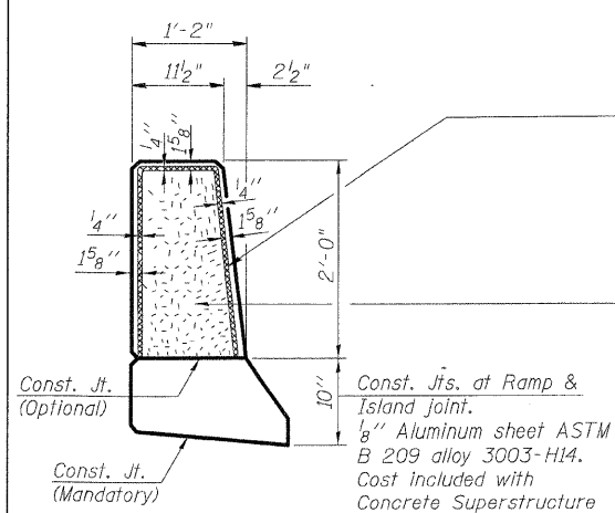
EXPANSION JOINT AT PARAPET DETAIL
