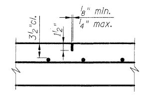
SAWED CONTRACTION JOINT DETAIL
