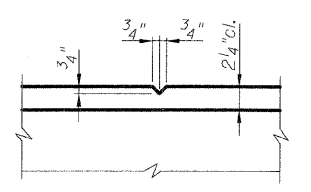
GROOVE JOINT DETAIL
