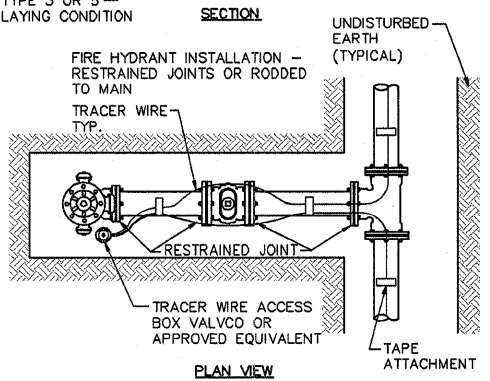
2 HYDRANT DETAIL 4 NOT TO SCALE
