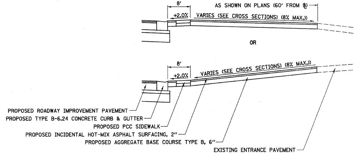
CROSS SECTION
