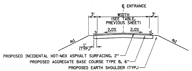
TYPICAL SECTION
