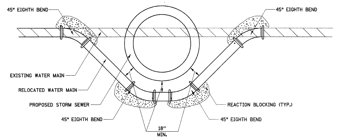
DETAIL OF LOWERING WATERMAIN
