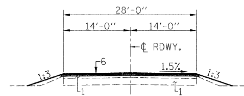
TYPICAL SECTION LUCAS STREET
