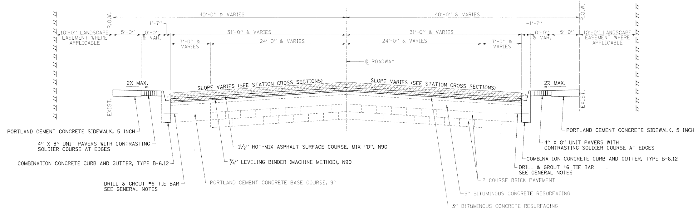
PROPOSED TYPICAL ROADWAY CROSS SECTION STA. 78+04.07 TO STA. 87+88.60
