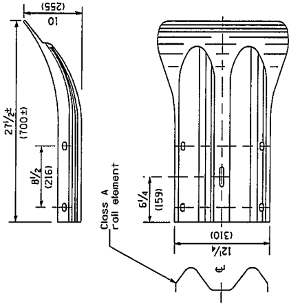
END SECTION
