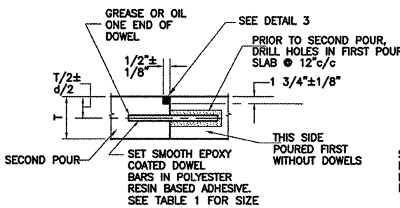
TYPE D - DOWELED CONSTRUCTION SYMBOL [Symbol]
