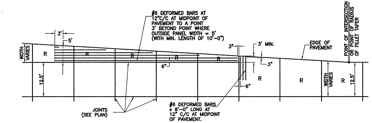
FILLET TAPER DETAIL
