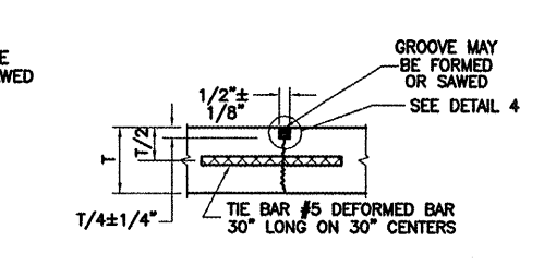
TYPE G - HINGED CONTRACTION SYMBOL [Symbol]
