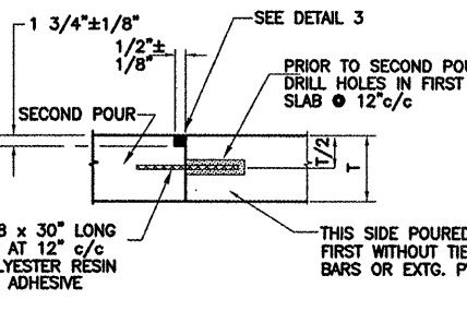
TYPE E-1 - HINGED WITHOUT KEY SYMBOL [Symbol]
