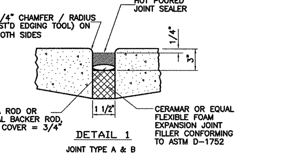
DETAIL 1 JOINT TYPE A & B
