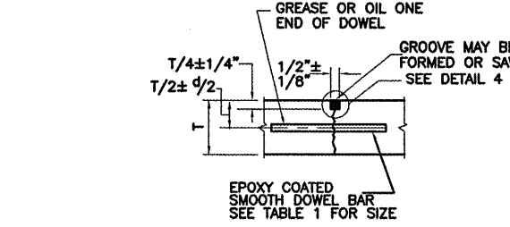
TYPE F - DOWELED CONTRACTION SYMBOL [Symbol]
