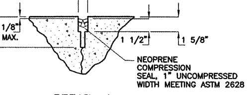
DETAIL 4 JOINT TYPES F, G, AND H
