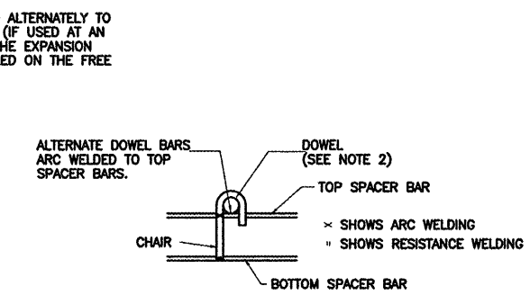
DOWEL BASKET ASSEMBLY DETAILS AND NOTES
