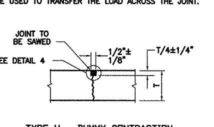
TYPE H - DUMMY CONTRACTION SYMBOL [Symbol]
