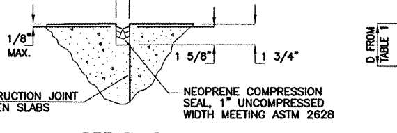
DETAIL 3 JOINT TYPES C, D, AND E
