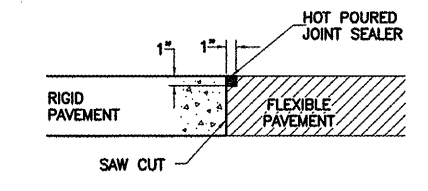
DETAIL - JOINT BETWEEN FLEXIBLE AND RIGID PAVEMENTS
