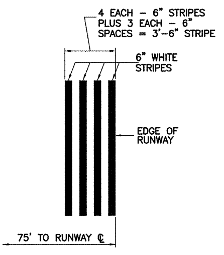
DETAIL A RUNWAY EDGE STRIPES STRIATED
