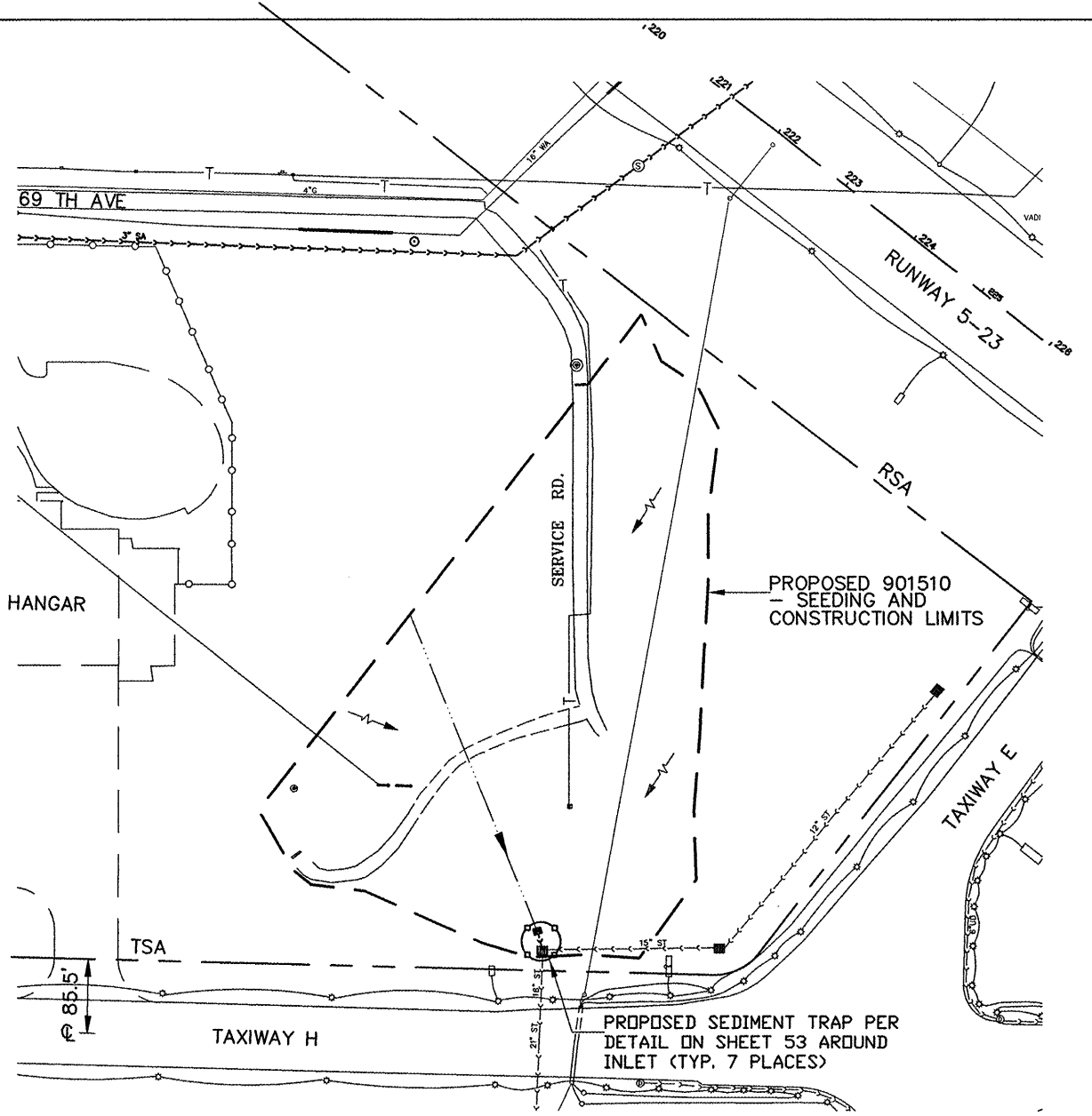
NORTH ON-SITE BORROW AREA PLAN
