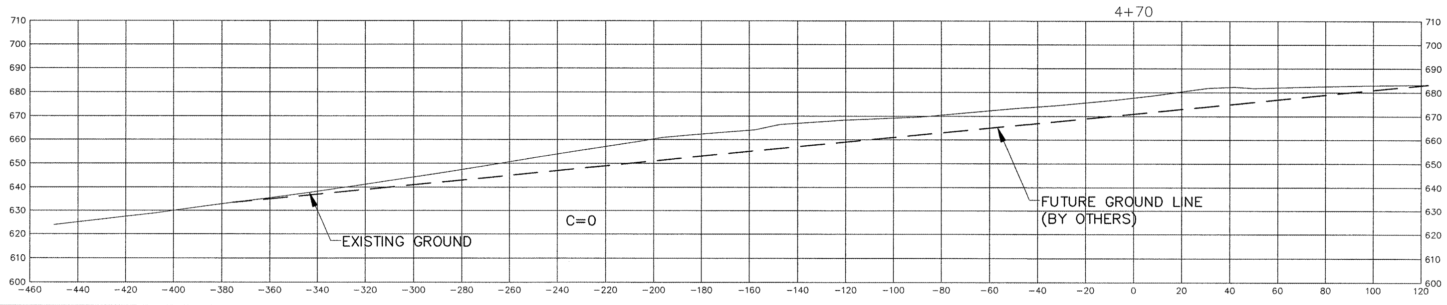
SOUTH OFFSITE BORROW EXCAVATION AREA, STA 4+70 TO STA 5+15
