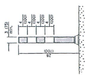
FLEXIBLE DELINEATOR
